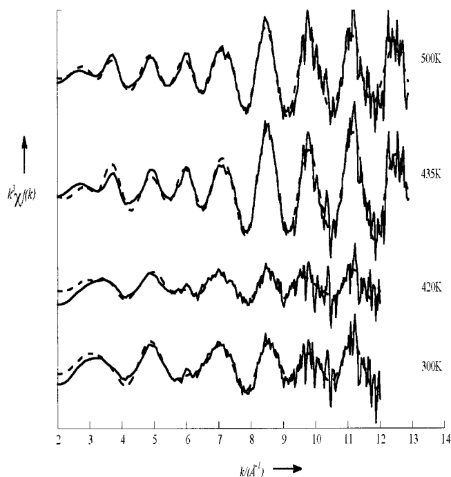
Figure 2. Representative k^3 -weighted EDE spectra derived during the reaction of 5 wt % Rh/ \gamma - Al_2O_3 catalysts for a reaction of a feedstock of composition NO/H_2/He = 1/3/96 at the temperatures indicated. Each spectrum (solid line) is acquired in 500 ms. The dashed line is the theoretical fit derived from an explicit analysis by using EXCURV 98.
